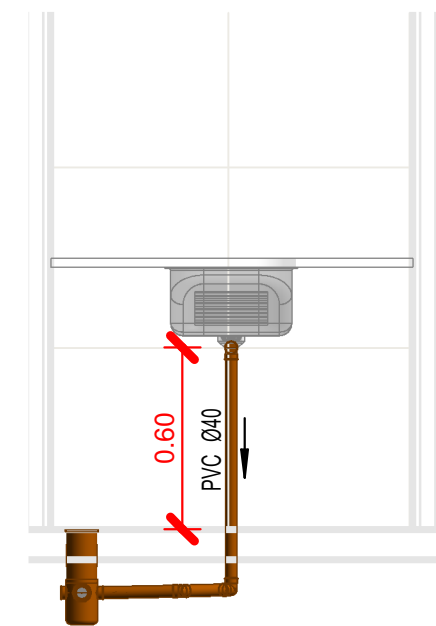
VISTA 04' - ESGOTO
